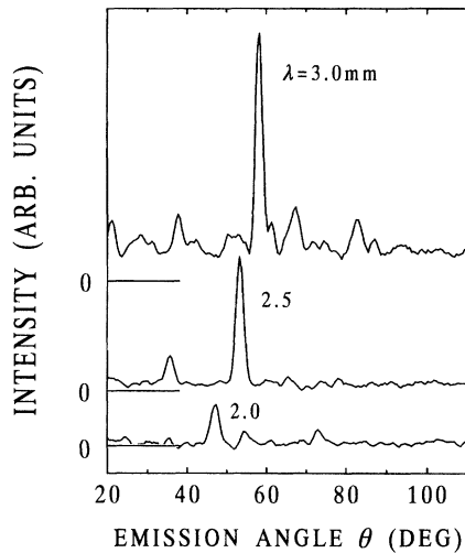
FIG. 2. Dependence of the coherent SPR intensity on the emission angle \theta . The intensity was measured with the 42 MeV short-bunched electron beam passing over a 6 mm period grating at the wavelengths 2.0, 2.5, and 3.0 mm.
